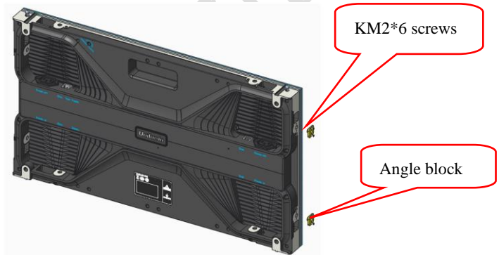
Fig 2-16 Installing angle block 1
