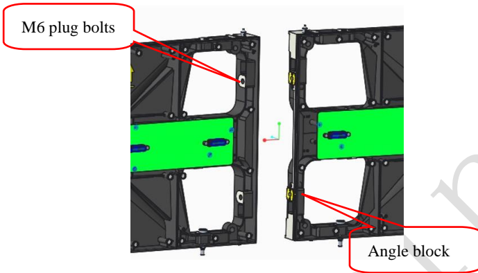
Fig 2-18 Splicing of left and right cabinet
