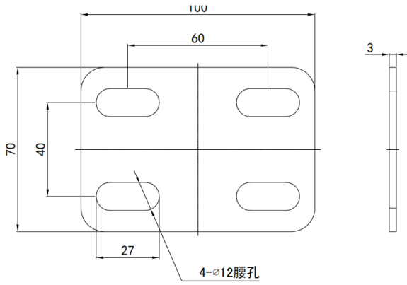
Fig 2-21 Rear Mounting Plate
