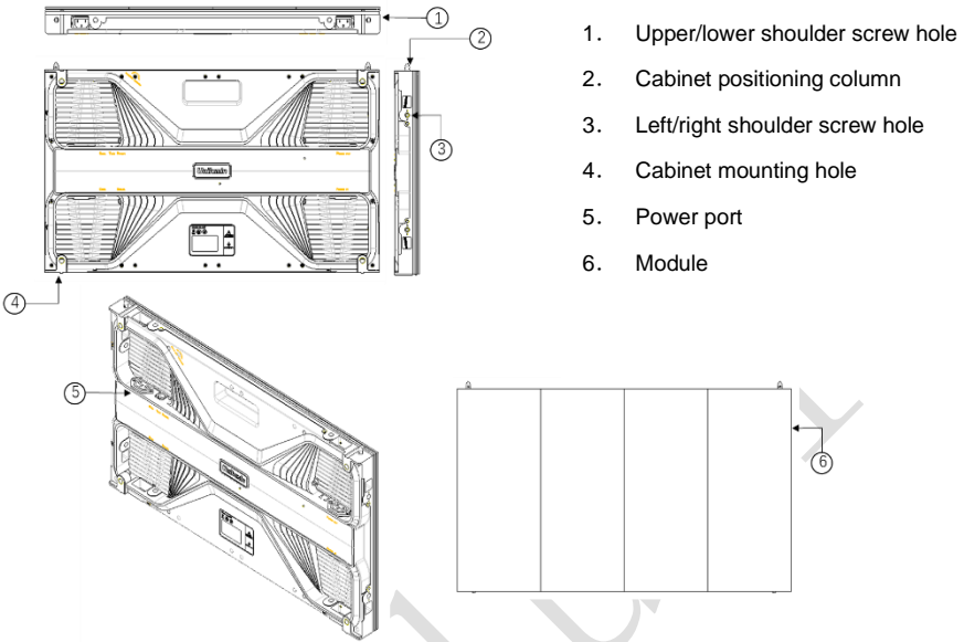
Fig 1-1 Cabinet Appearance
