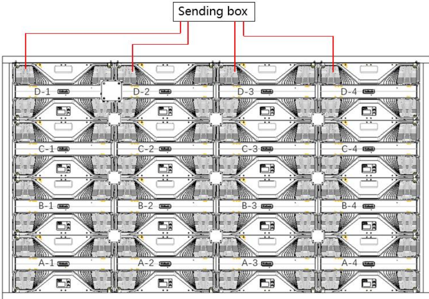
Fig 2-26 Signal Cable Connection Diagram of ULWIII 1.2
