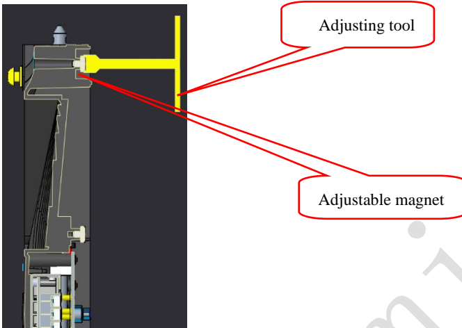
Fig 2-25 Schematic diagram of module flatness adjustment
