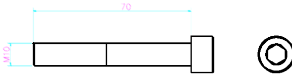
Fig 2-14 Rear installation M10x70 Inner hexagon bolt
