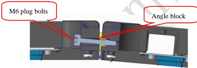
Fig 2-19 Internal drawing of left and right cabinet splicing
