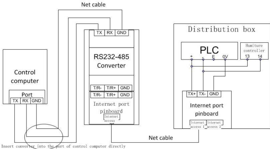
Fig 2-29 Distribution Box PLC Connection Diagram
