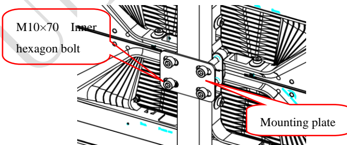
Fig 2-15 Back view of rear maintenance Installation Details
