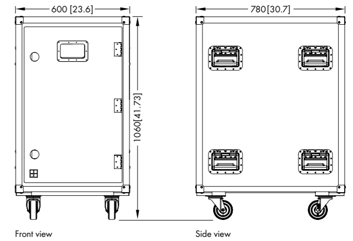
Front view Side view Z5576 D80 Touring rack assembly dimensions in mm [inch]
