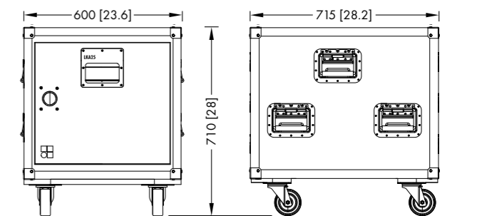
3 x D80 Touring rack dimensions in mm [inch]
